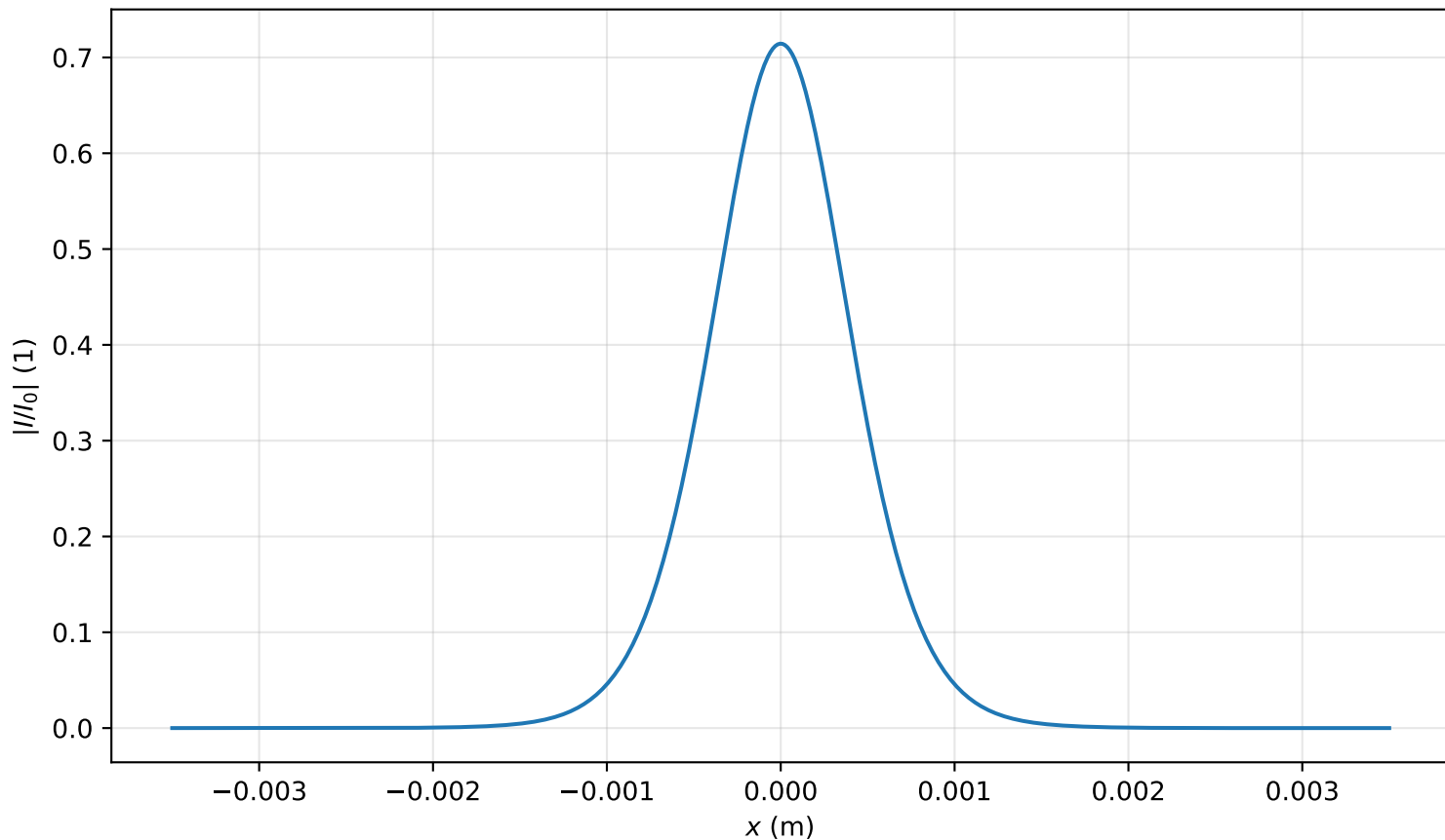
Intensity profile I(x, y = 0, z = 2.388m)/I_0 , P_{in}=0.5P_{cr} , artificial time
